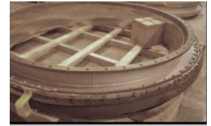
Figure 26 - Fully Assembled Expansion Compensator
